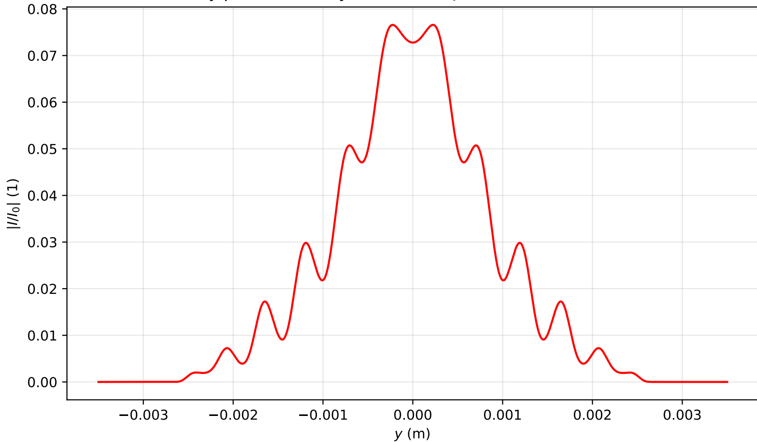
Intensity profile I(x=0, y, z=3.025)/I_0 , P_{in}=2.0P_{cr} , artificial time
